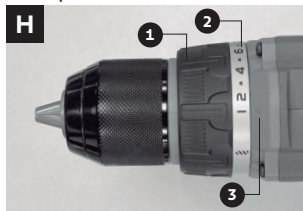
Figure H 1. Adjustment ring 2. Graduation 3. Arrow
